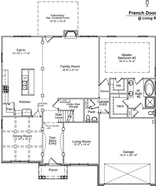
"A" 1st Floor Plan
