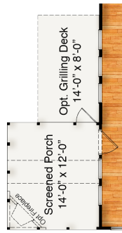
Optional Screened Porch
